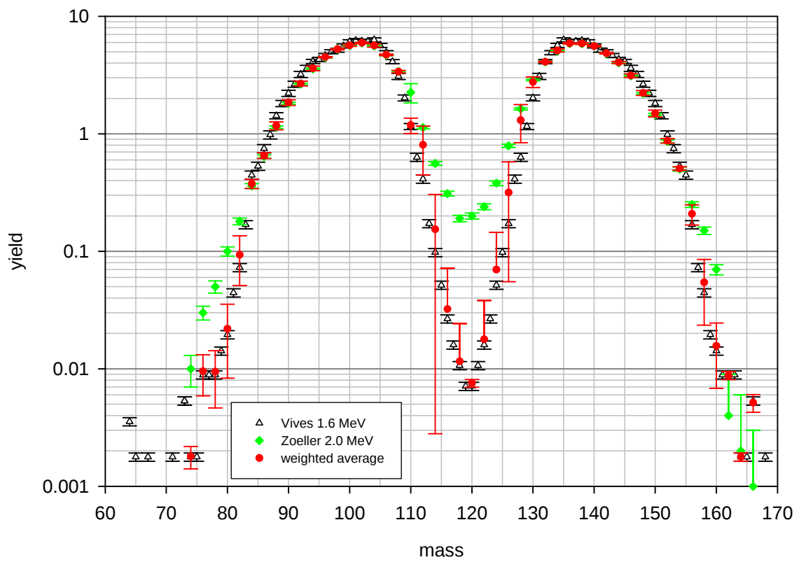
Benchmark A: ^{238}\text{U} at 1.6-2 MeV pre neutron emission experimental yields
